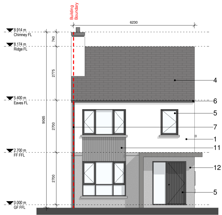
1 01 Front Elevation 1 : 100 @ A3
