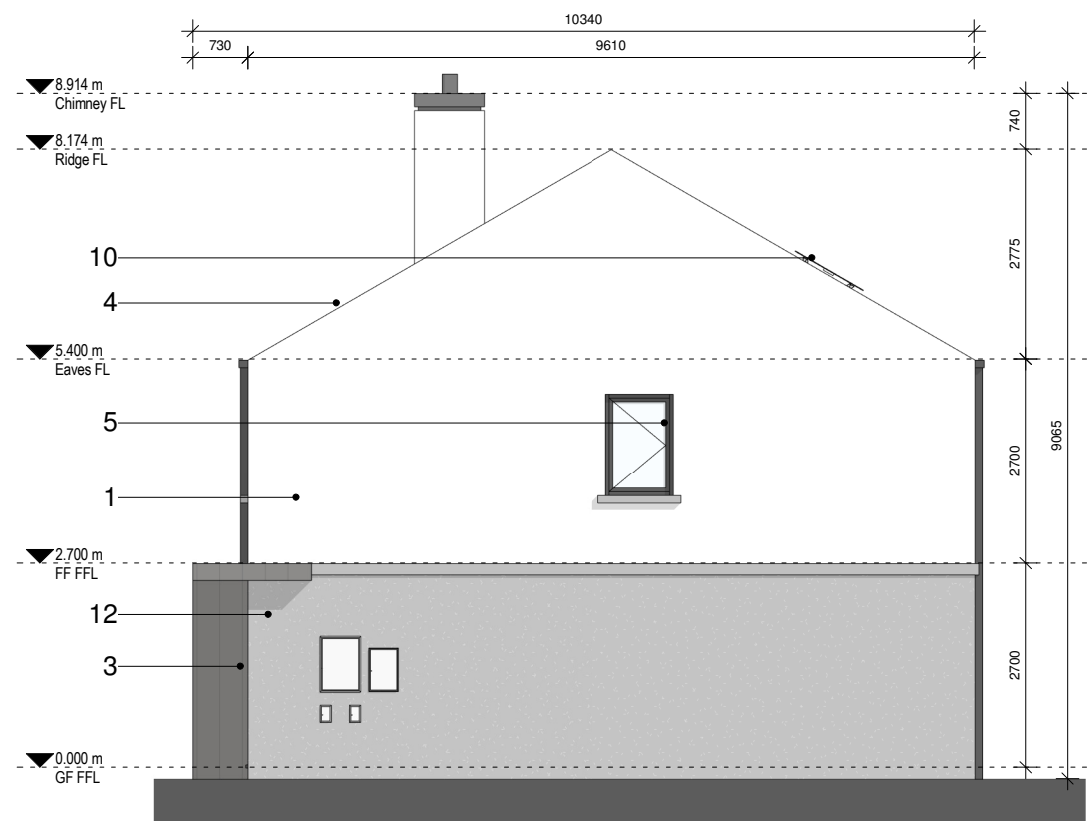
4 01 Side Elevation 1 : 100 @ A3
