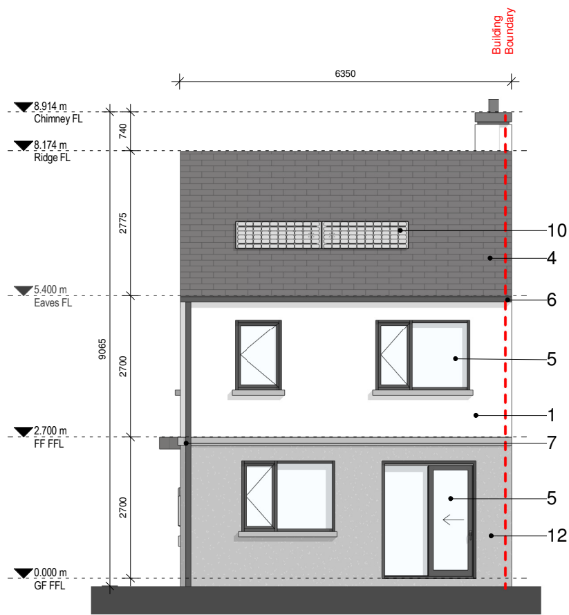
3 03 Rear Elevation 1 : 100 @ A3
